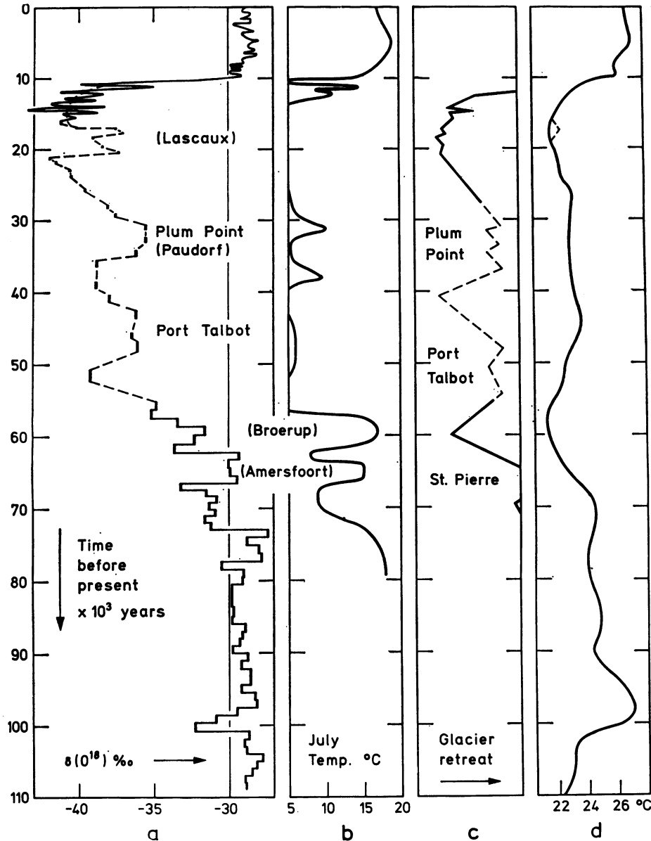
Fig. 5. Climatic variations during the last 70,000 or 100,000 years estimated by various methods. (a) The \delta(O^{18}) variations in the Camp Century ice core. (b) A C^{14} -dated pollen study from Holland (23). (c) A C^{14} -dated stratigraphic study of Pleistocene deposits in the Ontario and Erie basins showing the measurements of the edge of the Laurentian ice sheet (24). (d) An oxygen-isotope study on deep-sea cores showing part of a generalized temperature curve for the surface water of the central Caribbean (25). The dashed part of the curve is added by the present authors in view of the data given in (21). Dates established by C^{14} and Pa^{231}/Th^{230} . A 13,000-year climatic cycle is suggested. European names of interstadials are given in parentheses.
